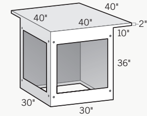
90° Corner Cabinet with 10" Cantilever on Two Sides 30"D x 30"L x 36"H
