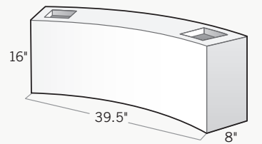
Curved Seating Wall (1/8 Circle) 8"D x 39.5"L x 16"H Curved seating wall is designed with a 51" radius from the center point to the inside edge, perfect for pairing with our round fire pit.
