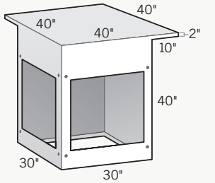
Bar-Height 90° Corner Cabinet with 10" Cantilever on Two Sides 30"D x 30"L x 40"H
