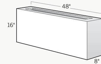
Straight Seating Wall 8"D x 48"L x 16"H Create seating walls in hours vs. days. Finish with Eldorado Stone & Wall Caps for an authentic masonry appearance.
