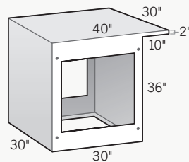
Cabinet with 10" Cantilever Backside 30"D x 30"L x 36"H
