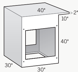
Bar-Height Cabinet with 10" Cantilever Backside 30"D x 30"L x 40"H
