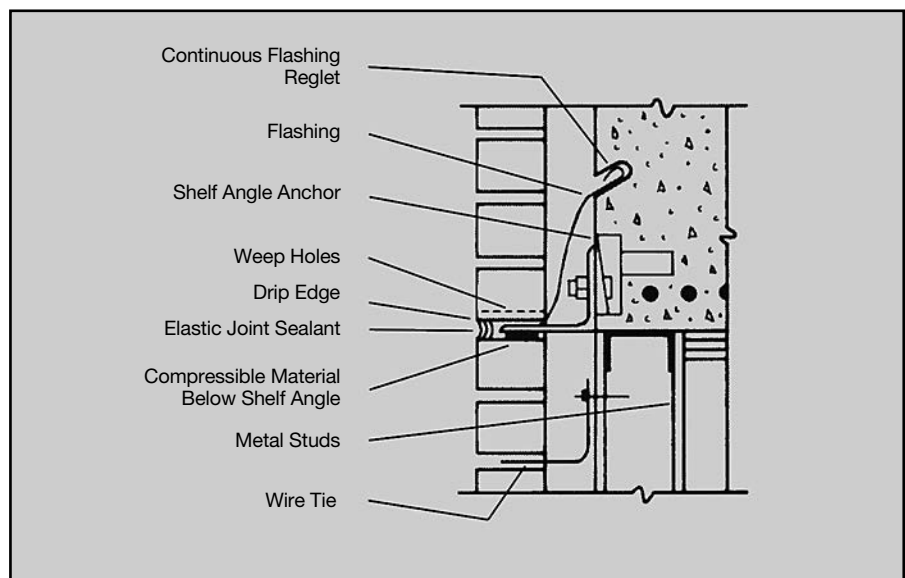
Horizontal Movement Joint at Shelf Angle
