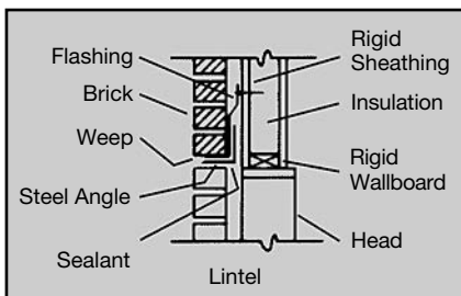
Typical Lintel and Sill Details
