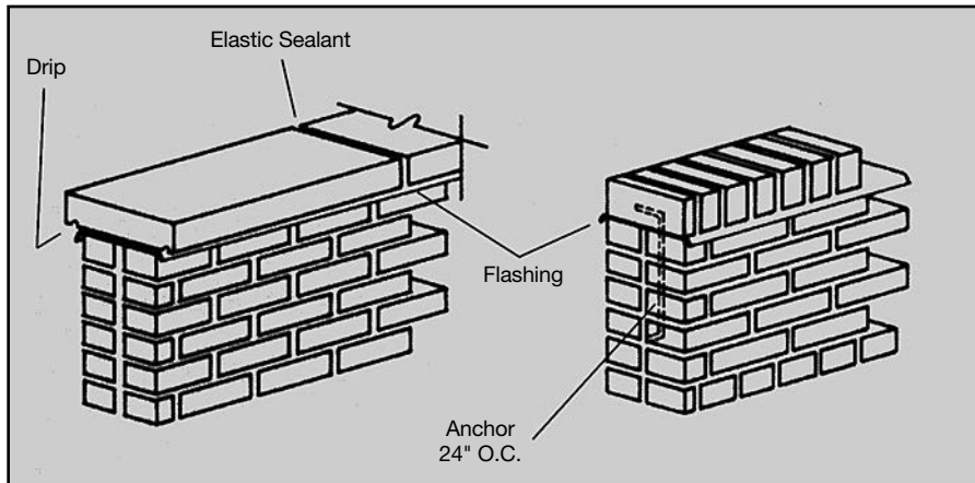
Stone Coping
