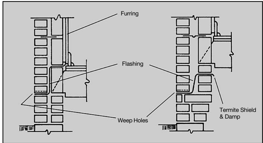
Flashing at the Bases of Masonry Walls
