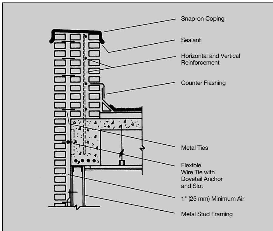
Reinforced Parapet Wall
