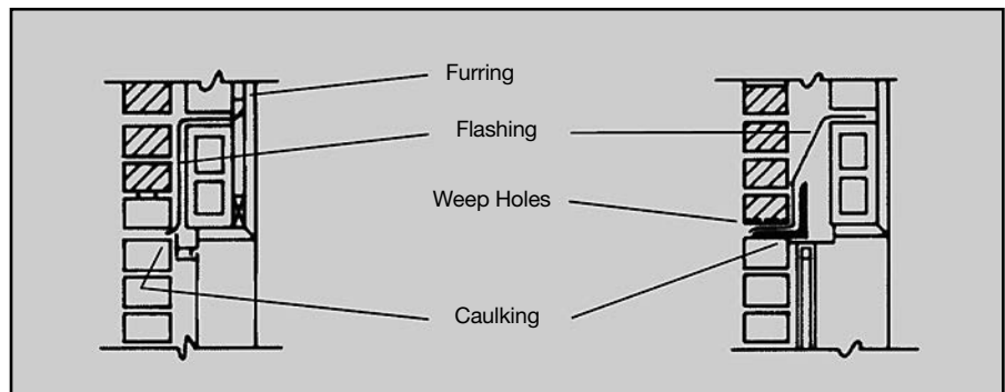
Flashing Heads of Openings
