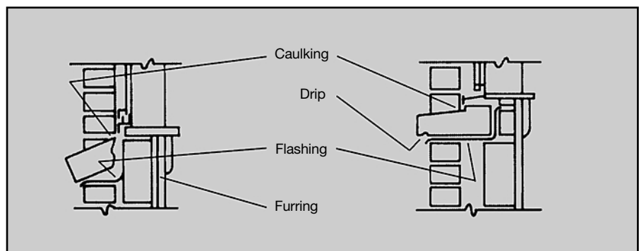
Flashing at Window Sills
