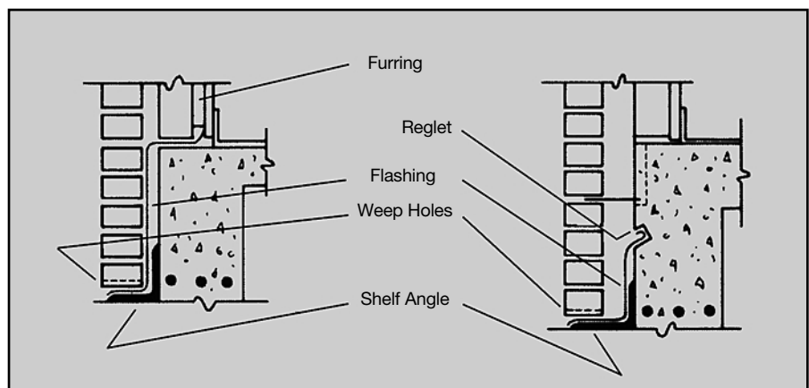
Spandrel Flashing
