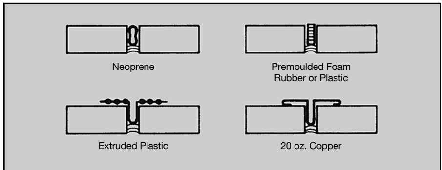
Movement Joint Fillers
