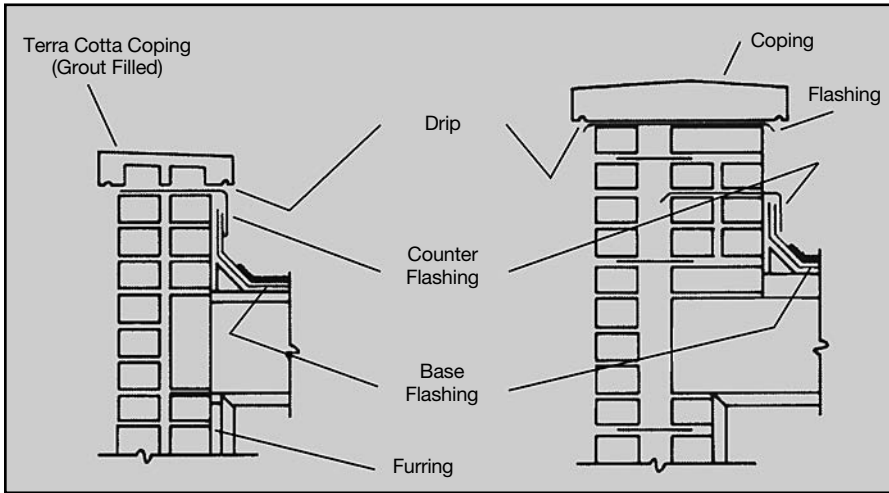
Flashing Copings of Parapet Walls
