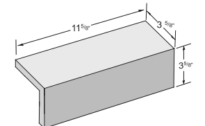
Utility Edge Cap 3 5/8" x 3 5/8" x 11 5/8"
