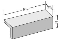
King Edge Cap 2 5/8" x 2 3/4" x 9 5/8"
