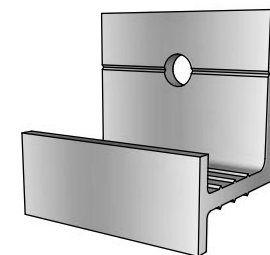
TIER® Kerf Bracket Mechanical Fixing Method Stainless Steel Fasteners Required
