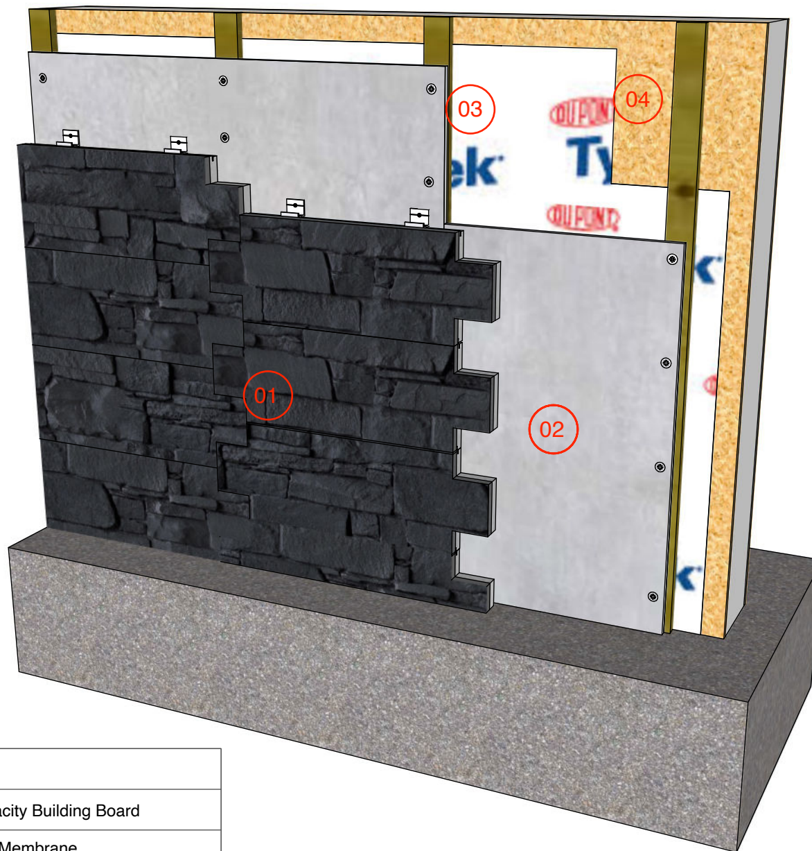
TIER® Kerf Bracket Mechanical Fixing Method. Stainless Steel Fasteners Required
